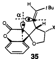
Figure 3. Proposed transition-state for the formation of 25 and 27 illustrating the optimal geometry for the manifestation of conformational memory effects.
