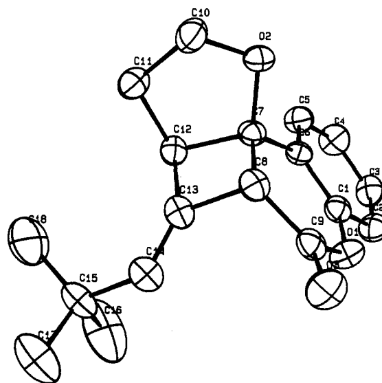
Figure 2. X-ray crystal structure of the photoadduct 25 .
