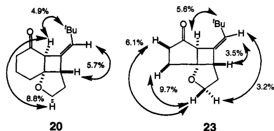
Figure 1. Representative ^1\text{H} NMR NOE data for photoadducts 20 and 23 .
